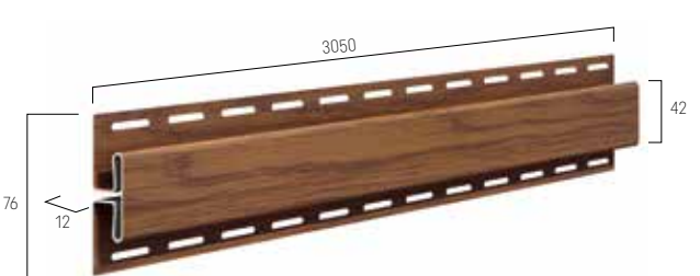
SV(P) 18 Connector
